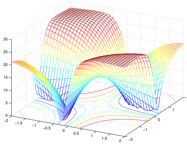
Fig. 2. Projection of the real pseudozero set of P_2
