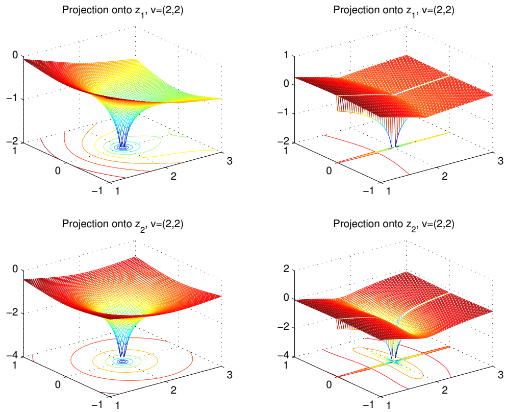
Fig. 1. Projections of the complex pseudozero set (on the left) and the real pseudozero set (on the right) of P_1
