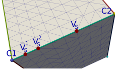
Figure 5: Conic cut.
